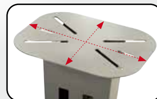
Plateau 4 trous oblongs de fixation 4 hole oblong fixing tray 380x300 mm
